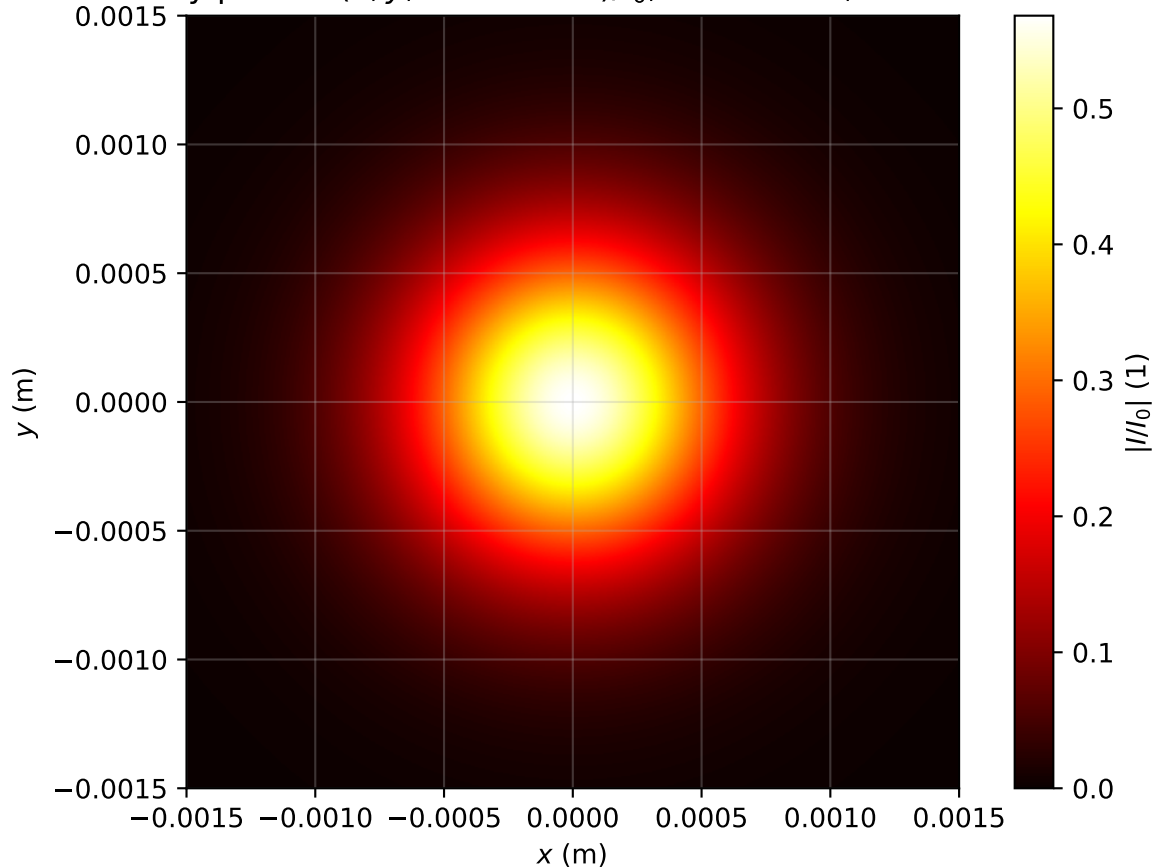
Intensity profile I(x, y, z = 3.503m)/I_0 , \text{Pin}=0.6\text{Pcr} , artificial time
